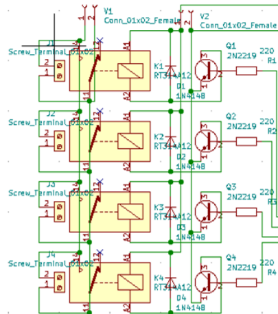
Figure 33. Relay Circuit Schematic
