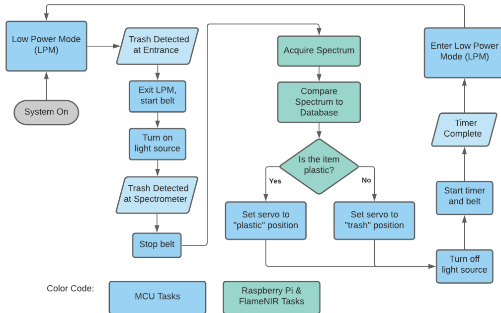
Figure 2. High-Level CAWSS Software Flowchart.
