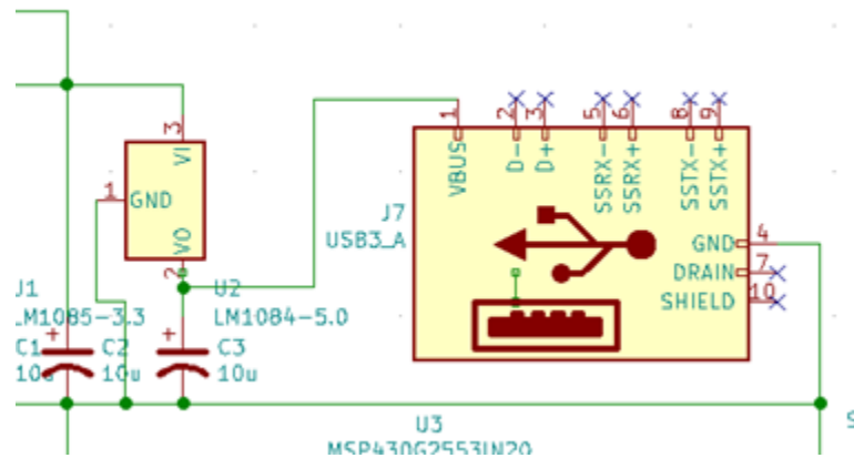
Figure 34. Spectrometer Driver Power Schematic
