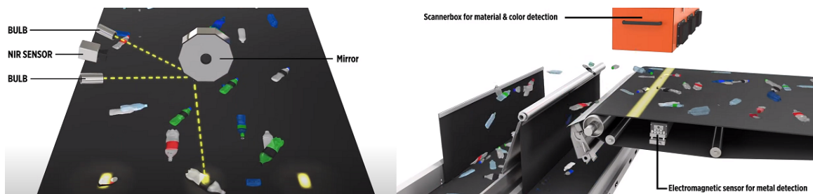
Figure 7. Tomra Automatic Waste Sorting System (Permission Pending)
