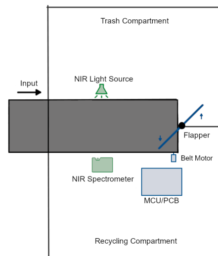
Figure 27. Internal CAWSS Diagram
