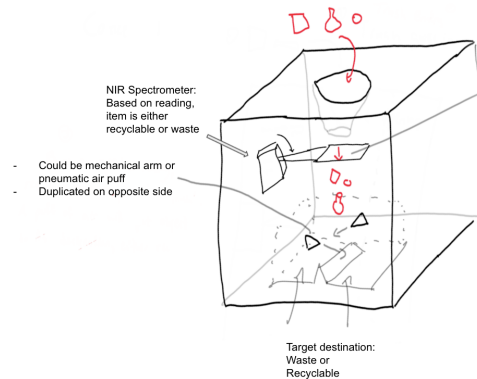
Figure 24. First Initial Design for CAWSS
