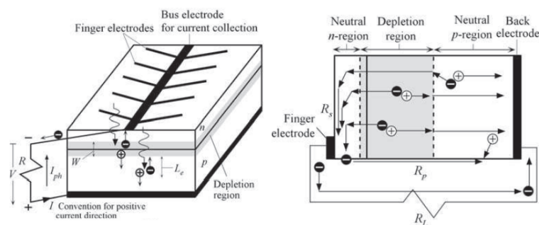
Figure 16. Function of a photovoltaic cell. Reproduced with permission from Optoelectronics and Photonics, 2nd Ed by Safa Kasap.
