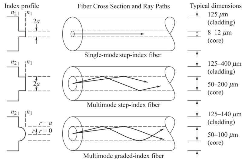
Figure 10. Diagram of step-index and graded-index fiber profiles. Reproduced with permission from Optical Fiber Communications, McGraw-Hill, 4th edition by Gerd Keiser
