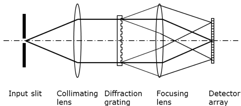
Figure 11. Traditional Spectrometer Design. Reproduced with permission from Ibsen Photonics.
