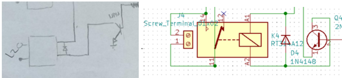
Figure 38. Hand Drawing Vs. Eeschema Part
