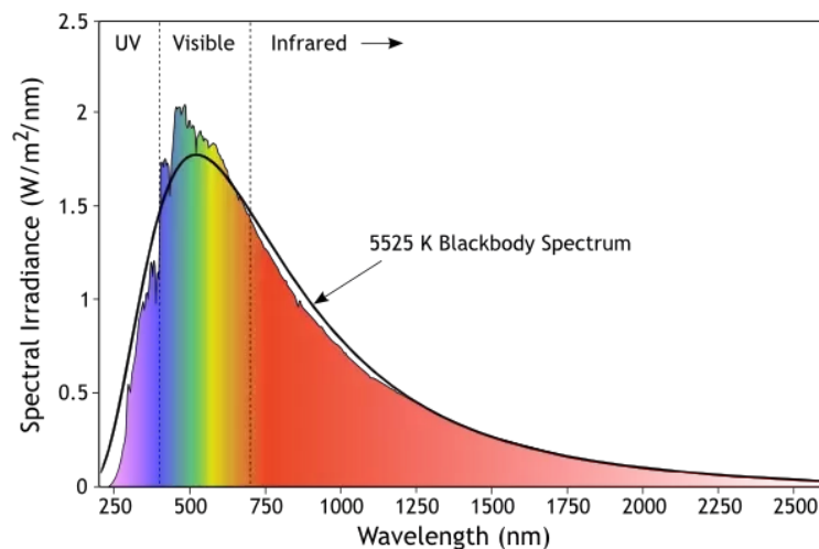
Figure 17. The sun's emission spectrum (permission pending)
