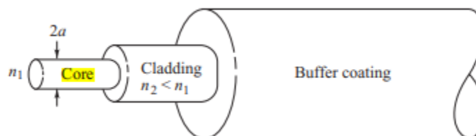
Figure 9. Anatomy of an optical fiber. Reproduced with permission from Optical Fiber Communications, McGraw-Hill, 4th edition by Gerd Keiser
