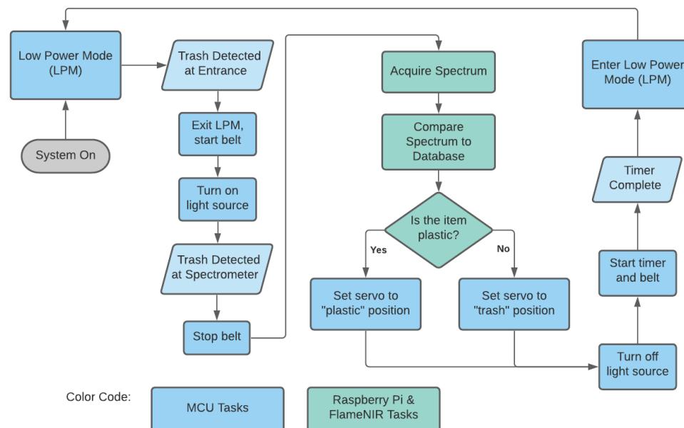
Figure 30. Generalized Software Architecture Flowchart
