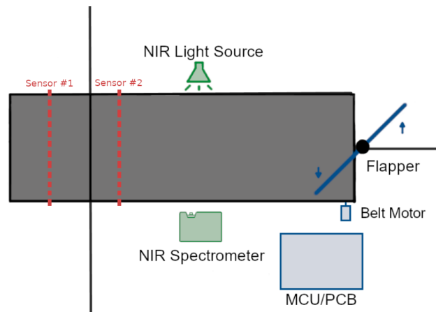
Figure 23. Diagram of Sensor #1 and #2 position
