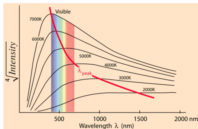
Figure 13. Visual representation of Wein's Law. Reproduced with permission from Rod Nave.
