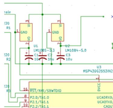
Figure 35. Microprocessor Power Schematic
