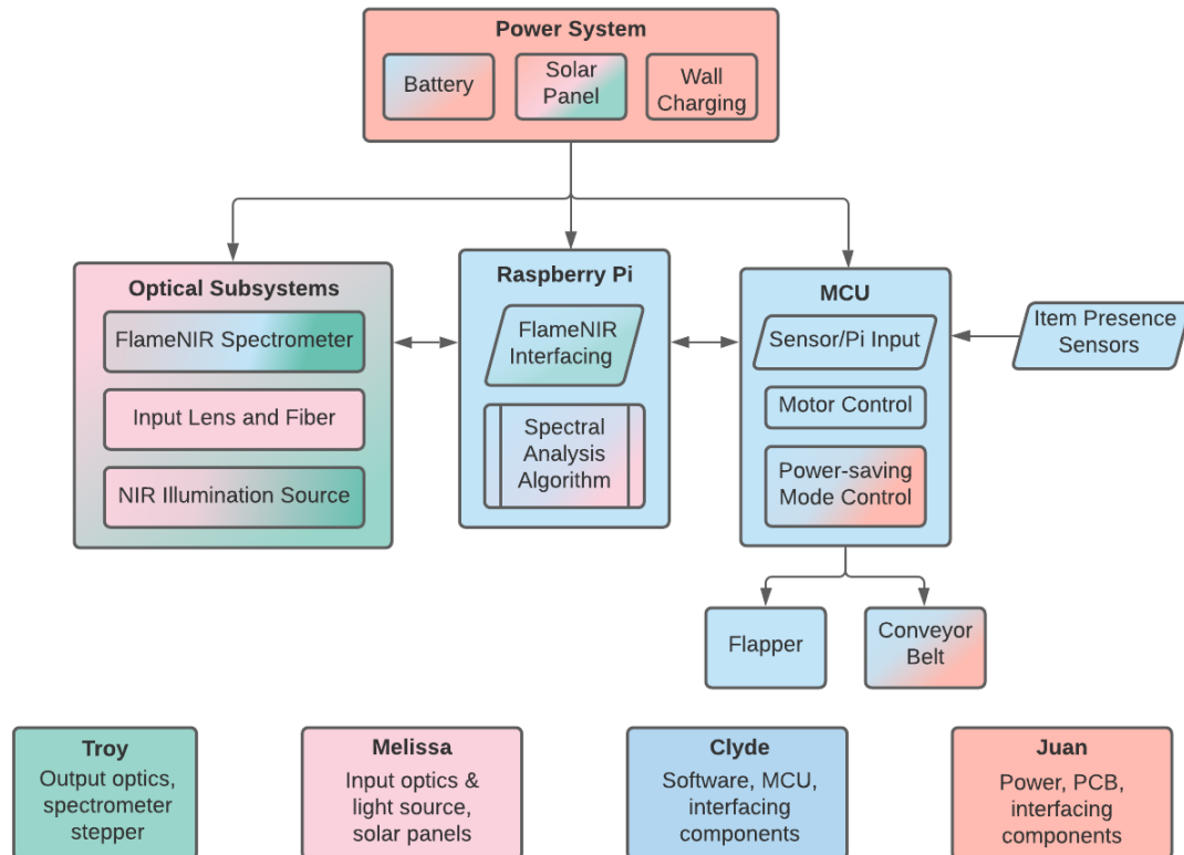
Figure 1. Generalized Flowchart for CAWSS Systems & Processes
