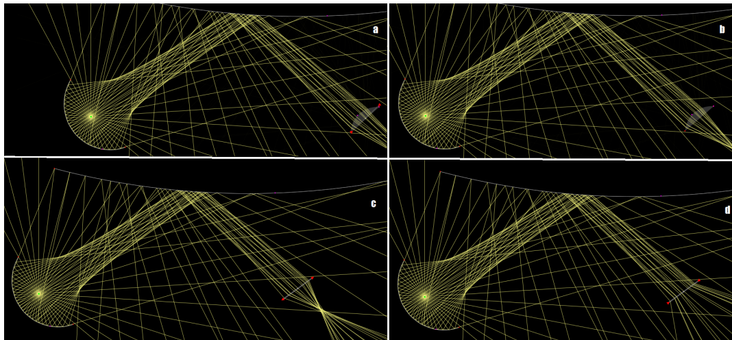
Figure 15. Ray traces associated with a) an achromatic doublet, b) a cylindrical lens, c) a convex lens, d) a concave lens.
