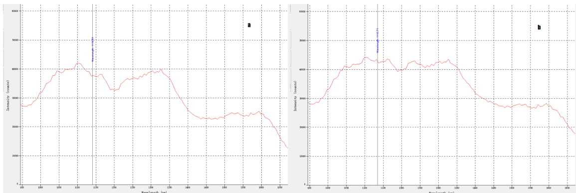
Figure 19. Nearly identical spectrums taken with a 250 W halogen of a) a known PET-G sample and b) a lid identified as a PET plastic.
