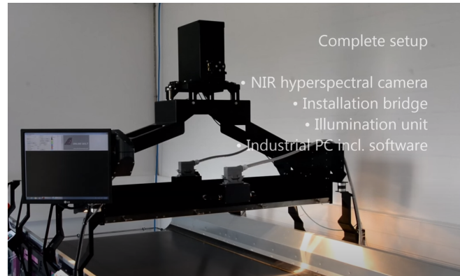
Figure 6. LLA KUSTA camera setup. Courtesy of LLA Instruments, Berlin
